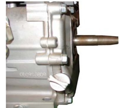
TAPERED CRANK
